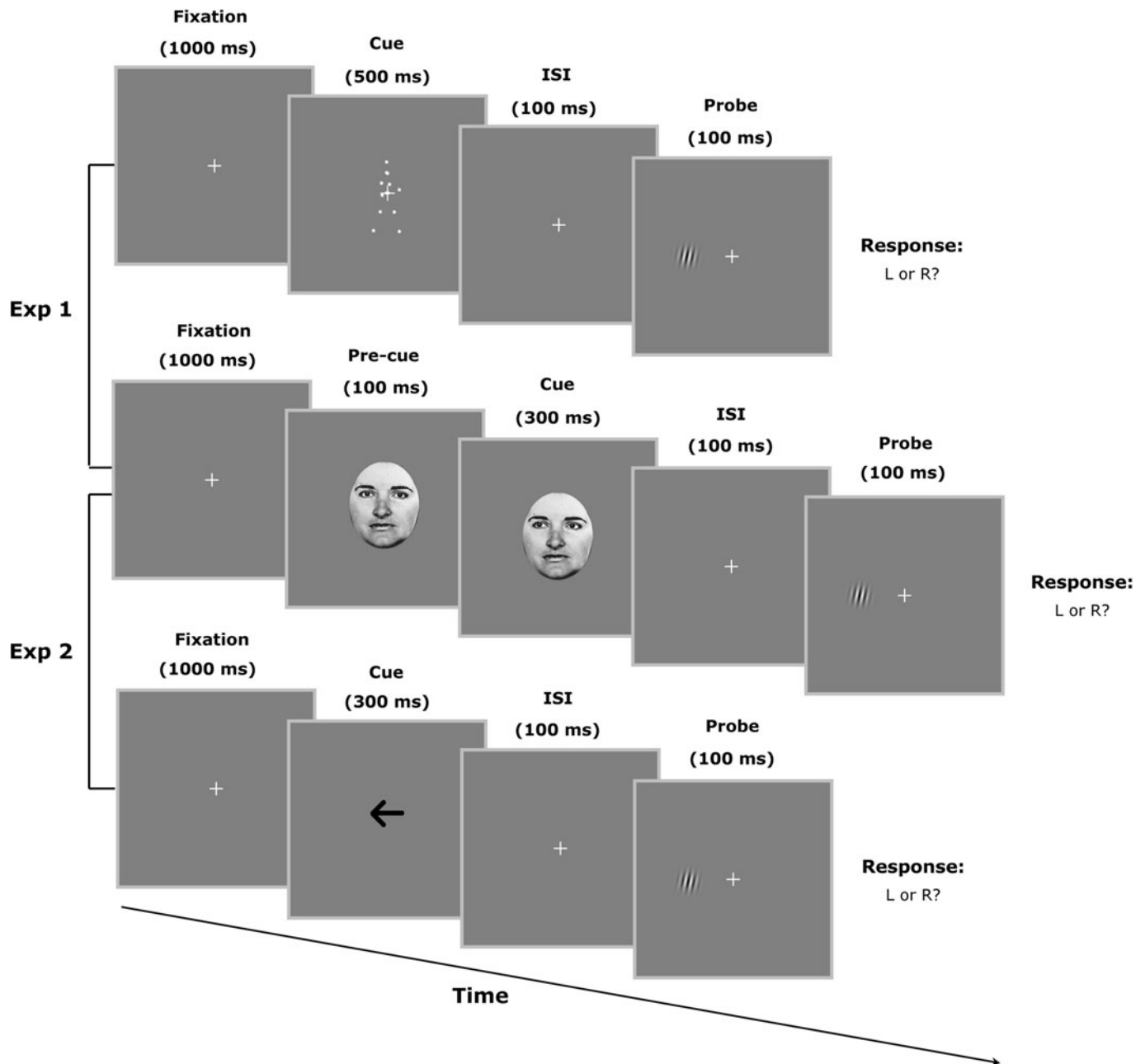
Fig. 1. Illustrations of trial sequences in the walking direction cueing, eye gaze cueing, and arrow cueing tasks. In the walking direction cueing task, after a cue (point-light BM stimuli with leftward or rightward walking direction) was presented for 500 ms in each trial, there was a 100 ms ISI in which only the fixation was displayed, followed by a small Gabor patch that was presented briefly (100 ms) as a probe on the left or right side of the fixation. Observers were then required to press one of two buttons to indicate whether the probe appeared on the left or right side as quickly as possible while minimizing errors. At the beginning of the task, observers were explicitly told that the walking direction was not predictive of target location. The procedure of the eye gaze cueing task was similar to that of the walking direction cueing task with the exception that faces with leftward or rightward eye gaze were employed as cues and they were presented for 300 ms. The arrow cueing task was identical to the eye gaze cueing task except that leftward or rightward arrows were used as cues.
